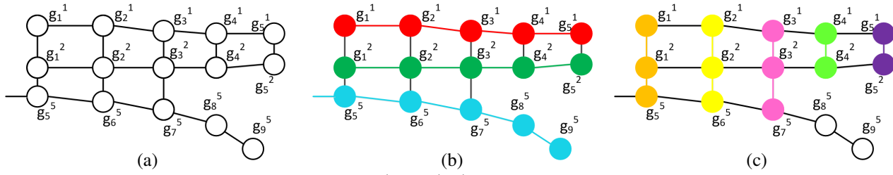
Figure 5. Illustration of our BCD inference. Note that g_i^j = (h_i^j, y_i^j) . (a) Graphical model consisting of 3 roads that have overlapping constraints ( i.e. , vertical edges). We alternate between performing inference (b) over each road one at a time (red, green, blue), and (c) along chains on the vertical direction encoding the horizontal constraints, also one at a time (orange, yellow, pink, green, purple). Note that these operations involve conditioning, and thus the pairwise potentials between a variable in the chain and a connected variable not in the chain are folded as unaries.
