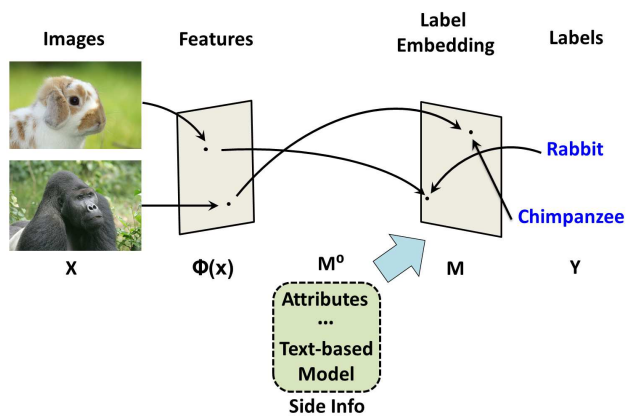
Figure 1: Illustration of the proposed framework. The model can automatically learn the label embeddings M , while side label information, denoted as M^0 , is optional.
