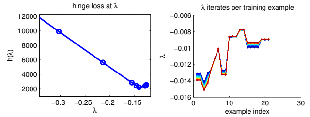
Figure 4. The convex function h(\lambda) sampled at breakpoints (left), and evolution of \lambda_n^{(\tau)} 's over time \tau (right). Warmer colors represent later iterations.
