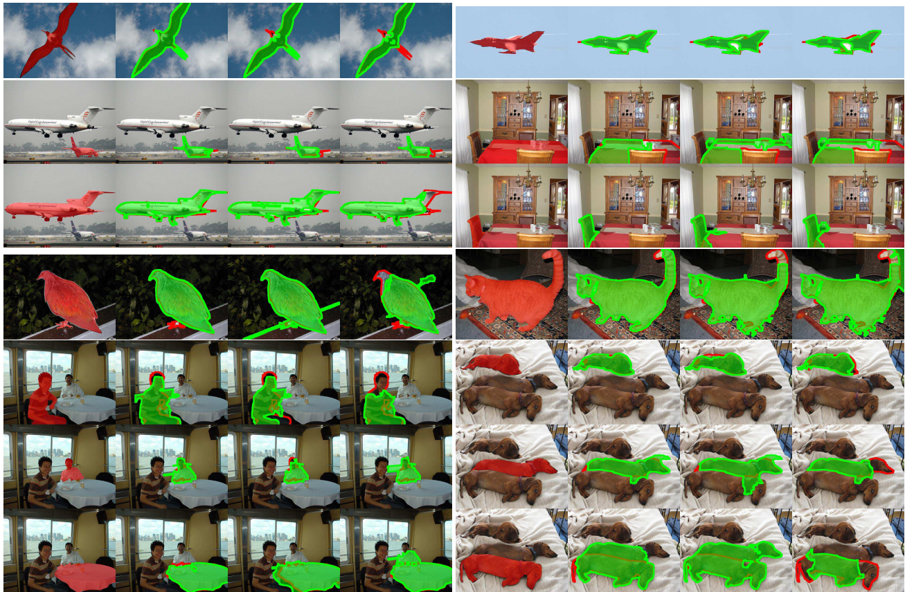
Figure 8. Example region proposals found for images from VOC 2012. Red masks denote ground truth, green masks denote the corresponding top proposals (from left to right).
