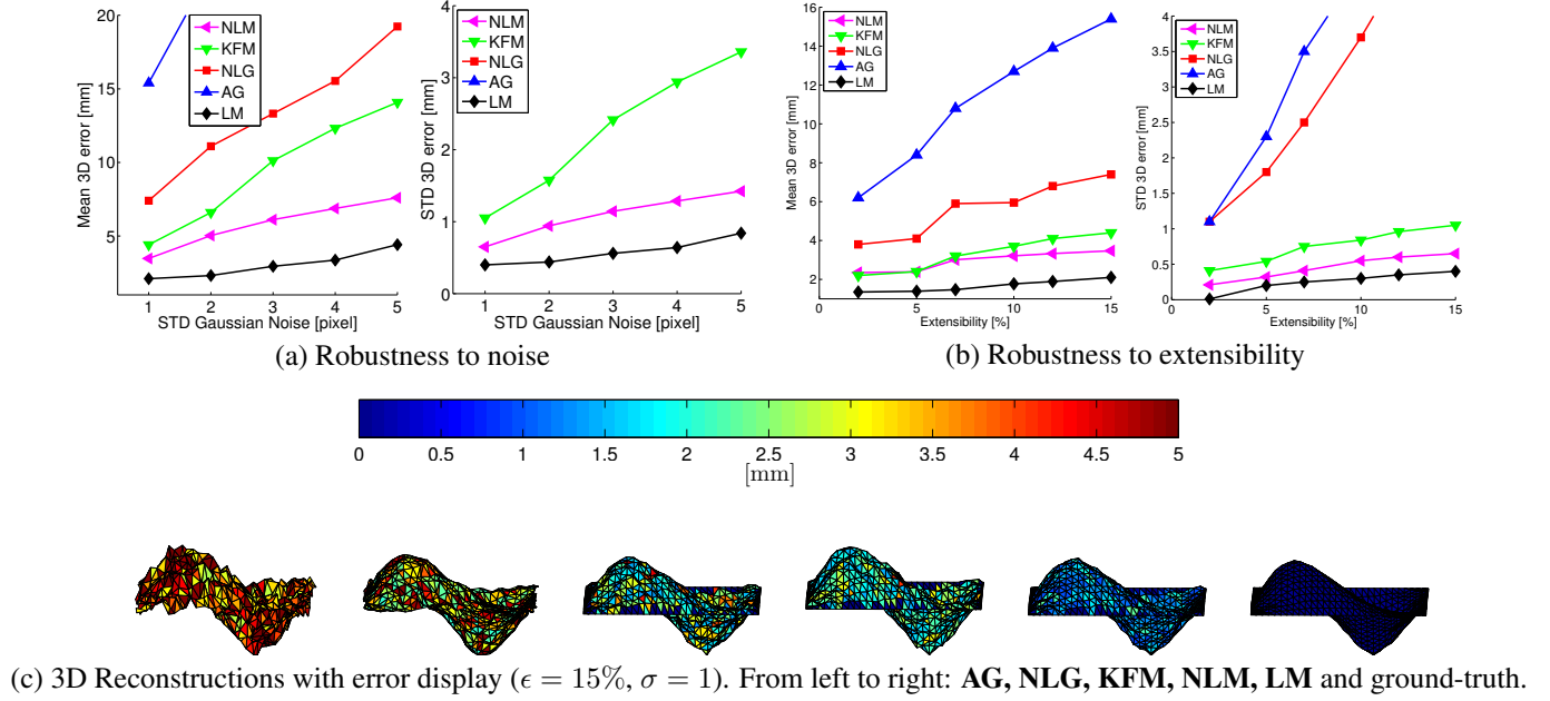
Figure 3. Results on simulated deformations. Large error results are not displayed to fit the error scale of the most accurate methods.
