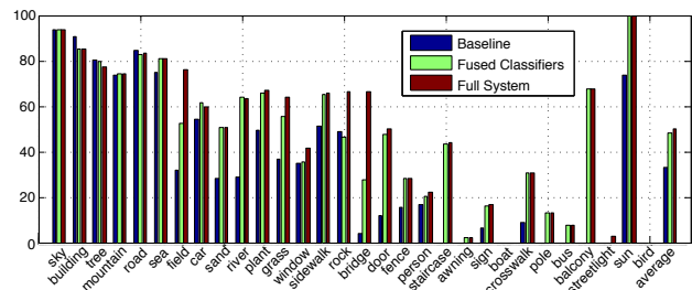
Figure 5. Classification rates (%) of individual classes for the baseline, fused classifiers, and the full system on SIFTflow. Classes are sorted from most frequent to least frequent.
