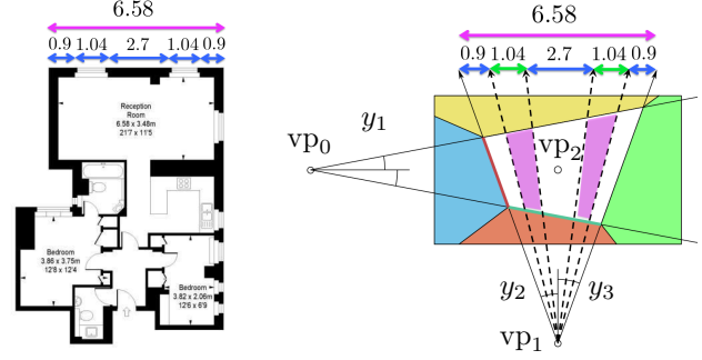
Figure 3. (Left) Example of a floor-plan with window-to-wall ratios, (Right) The window-to-wall ratios in the floor plan enable us to compute the rays (dashed lines) for the windows given y_2 and y_3 in our layout problem. Windows are denoted with green lines.
