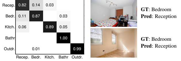
Figure 5. Left: Scene confusion matrix. Right: Examples of misclassification. Note that some cases are ambiguous since the room is empty and the annotator made use of the floor plan to label it.
