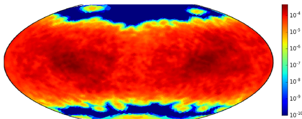
Figure 8: A Winkler-Tripel projection of the importance distribution of view directions, q^R , averaged over the thermus dataset at a typical iteration. Clearly visible is the equatorial belt of likely views, while axis aligned views (those on the top or bottom of the plot) are rarely seen.
