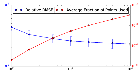
Figure 6: Relative error (blue, left axis) and fraction of total quadrature points (red, right axis) used in computing \log p(\tilde{\mathcal{I}}|\theta, \tilde{\mathcal{V}}) as a function of the ESS scaling factor, s_0 (horizontal axis). Note the log-scale of the axes.
