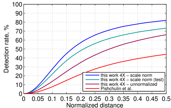
Figure 16: MPII - average PCKh for all joints
