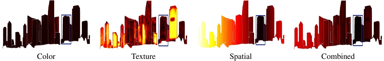
Figure 5: Figure shows color , texture , spatial models and the combined unary costs for a sample building (within the box) with \alpha = 0.35 and \beta = 0.4 . The regions with low costs are darker (black) than the ones with high cost (yellow). The corresponding image is the left skyline in Figure 8. (Note: images are costs, rescaled and resized for visibility.)
