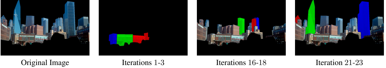
Figure 4: Progression of refined MRF algorithm for a sample image. In the first 3 iterations, three buildings are selected in the order, 1 st in red, 2 nd in green and 3 rd in blue color. Similarly, intermediate 3 and last 3 iterations are shown on the right.
