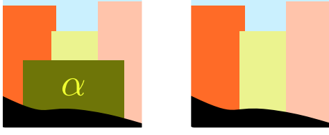
Figure 3: Given a label \alpha (left) one can infer the background labels underneath \alpha by copying the labels from the top to bottom because of the tiered structure (right).
