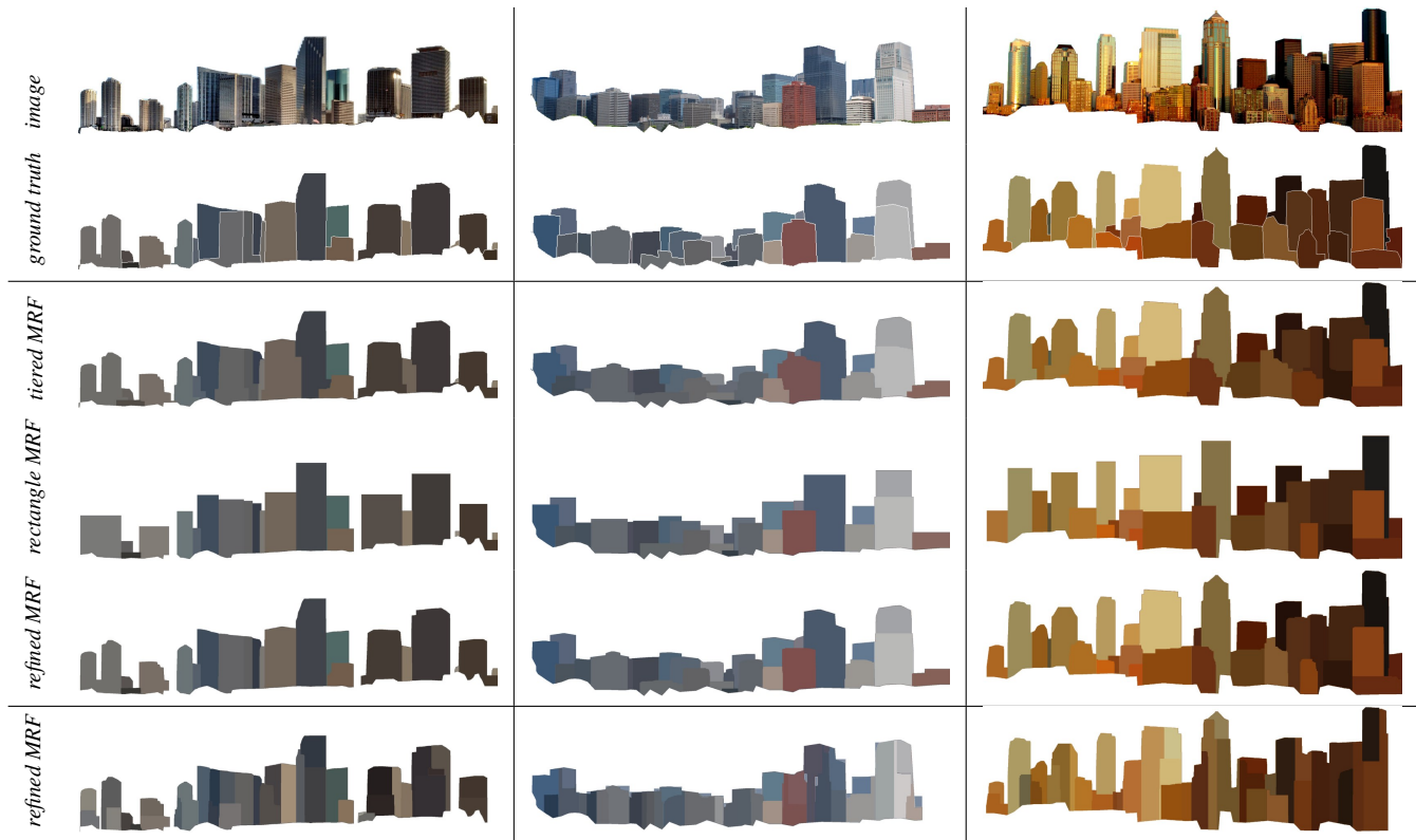
Figure 8: Skyline segmentation results for three images. In first and second row, original skylines within the upper and lower boundary and the corresponding ground truth segmentation are shown. In third, fourth, fifth and sixth row, outputs of the interactive tiered MRF , rectangle MRF , refined MRF and automatic refined MRF are shown respectively.
