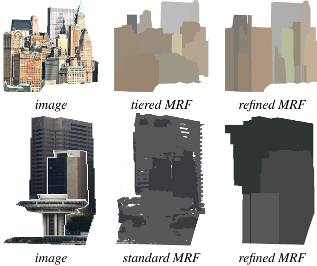
Figure 7: Some failures of the shape-constrained MRFs. On the image in the top row, the buildings are not rectangular and the refined MRF makes many mistakes, and the tiered structure alone is more appropriate. On the bottom row, the refined MRF incorrectly segments the concave buildings in the bottom.
