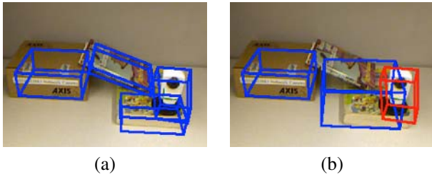
Figure 5. (a) Well fit boxes should not intersect much with neighboring boxes. (b) If two segments are merged incorrectly, e.g., the two books in the image, then the new box fit to the segment is likely to intersect with neighboring boxes, e.g., the box shown in red.
