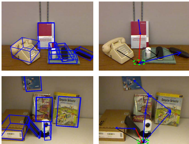
Figure 12. We qualitatively show our box fitting algorithm (left) on daily objects with ground-truth image segmentation and the supporting relation prediction after stability reasoning (right). Boxes for large surfaces (like the back wall and the ground) are not displayed for better visualization. The ground plane is plot as a green dashed circle for showing the support inference results.
