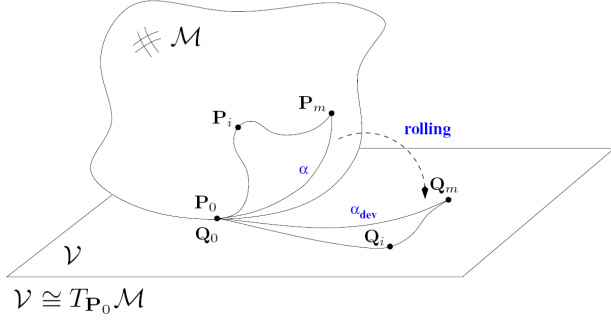
Figure 1. Rolling Map : \mathcal{M} rolls upon \bar{\mathcal{M}} = \mathcal{V} \cong T_{P_0}\mathcal{M} without slip or twist, along a rolling curve \alpha: [0, T] \rightarrow \mathcal{M} [22].
