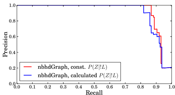
Figure 10: Precision-recall results on the KITTI 05 sequence, comparing the results using a constant value for P(\mathcal{Z}_q|\mathcal{L}_i) , and one which calculated P(\mathcal{Z}_q|\mathcal{L}_i) using the dataset ground-truth.
