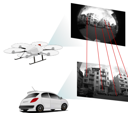
Figure 1: In an effort to move towards robust mapping and localization in unconstrained environments, this paper investigates graph comparison approaches to visual place recognition. Structural and visual information provided by covisibility graphs is combined, in order to cope with variations and noise in observations, such as those coming from heterogeneous teams of robots.
