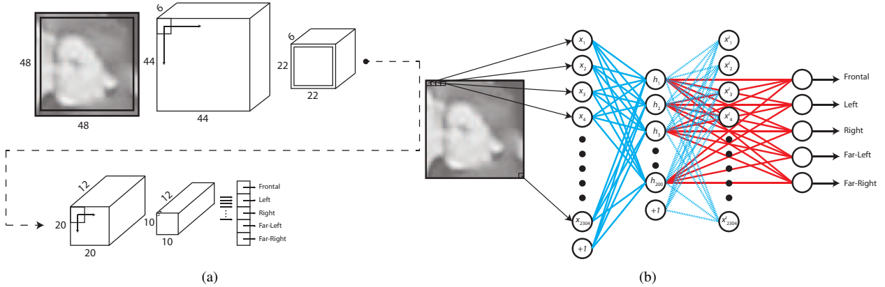
Figure 3. (a) Architecture of CNN. (b) SAE architecture: in cyan are pictured the interconnections between the auto-encoder that must be trained separately, in red instead there are the interconnections of the final NN.
