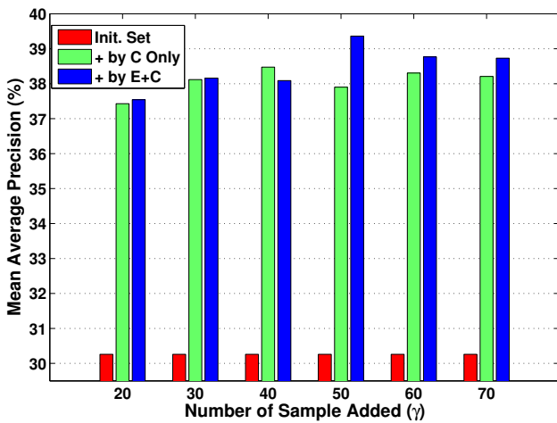
Figure 3. Mean average precision (mAP) of 11 category by our method varying the number of unlabeled images selected. The red, green and blue are the mAP using the initial labeled set (Init. Set), the augmented set by our method using category wide attributes only (+ by C only) and categorical+exemplar attributes respectively. (+ by E+C)
