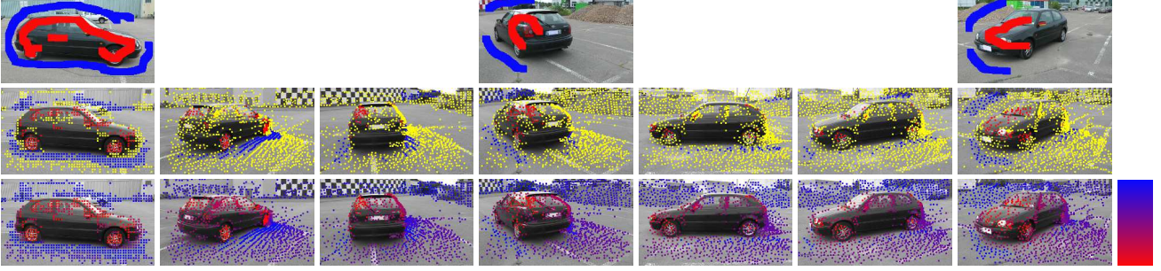
Figure 3. If we sparsely annotate a video over time and space (top row), the pre-computed trajectories propagate this information to other frames (middle row). Unlabeled trajectories (yellow) get a likelihood of object or background from a random walk computation [12] (bottom row). The likelihood is shown by a color that is a linear interpolation between red and blue as shown in the color bar. The strokes in just these three frames were the only user input for this video.
