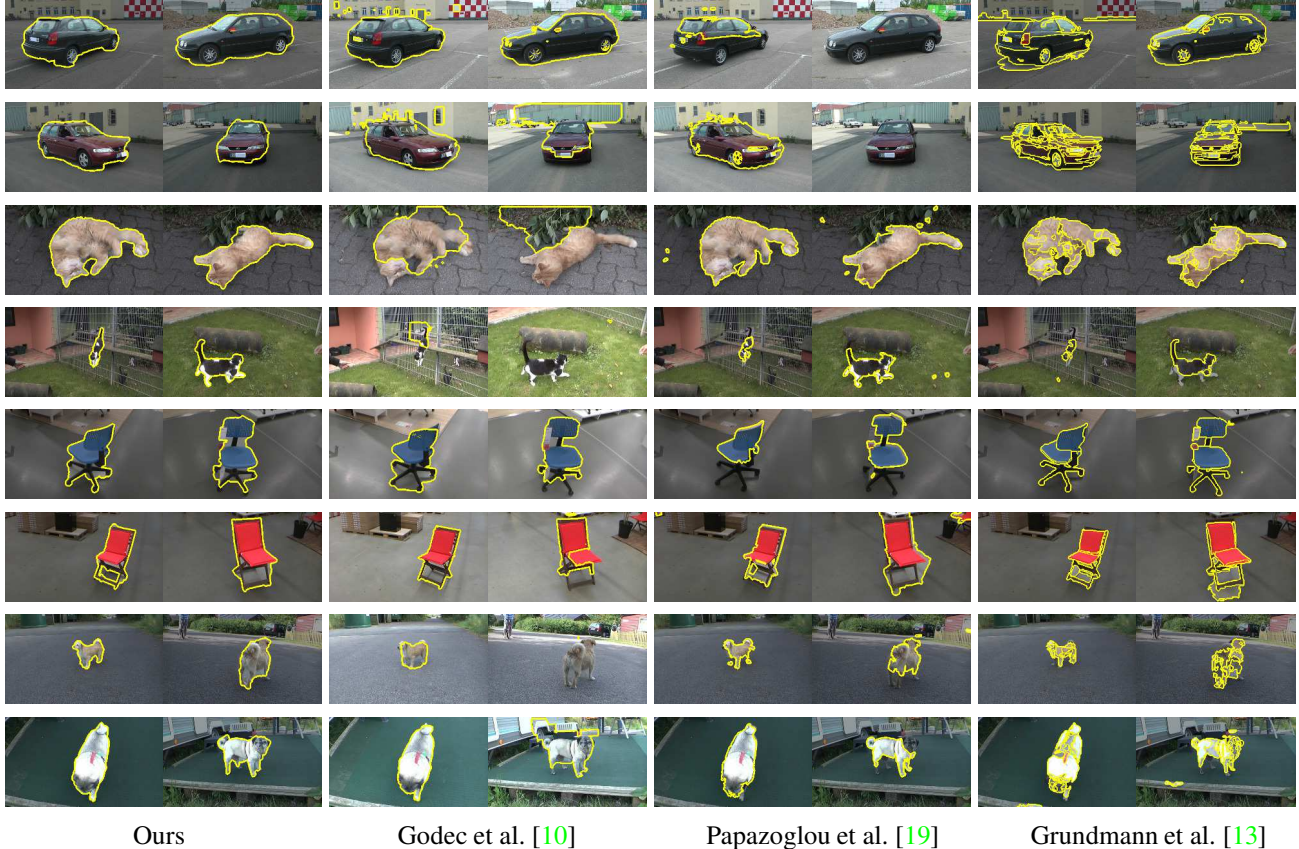
Figure 8. Qualitative comparison on car,cat,chair and dog videos for the output of the first iteration of user interaction for our method, [10], [19], and [13]. The foreground is highlighted with an yellow contour. An image with no foreground contour has an empty segmentation.
