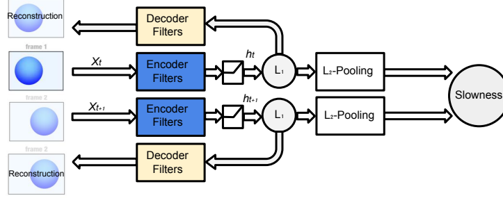
Figure 3: Block diagram of the Siamese convolutional model trained on pairs of frames.
