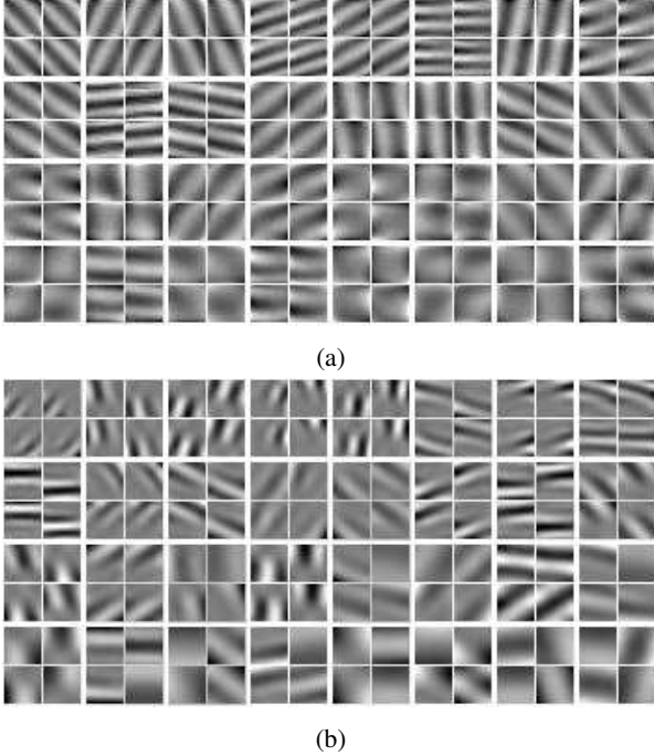
Figure 2: Pooled decoder dictionaries learned without (a) and with (b) the L_1 penalty using (2).
