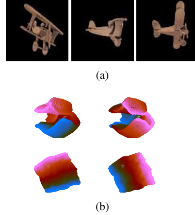
Figure 1: (a) Three samples from our rotating plane toy dataset. (b) Scatter plot of the dataset plotted in the output space of G_W at the start (top) and end (bottom) of training. The left side of the figure is colored by the yaw angle, and the right side by roll, 0^\circ blue, 90^\circ in pink.
