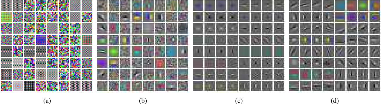
Figure 5: Pooled convolutional dictionaries (decoders) learned with: (a) DrLIM and (b) sparsity only, (c) group sparsity, and (d) sparsity and slowness. Groups of four features that were pooled together are depicted as horizontally adjacent filters.
