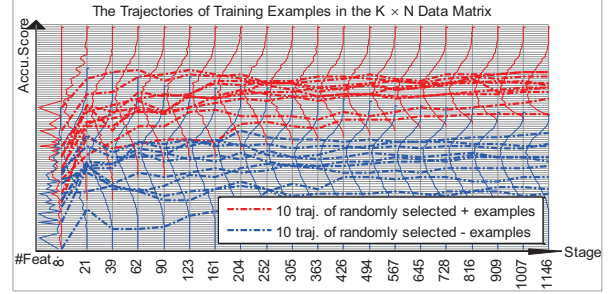
Figure 3. The K \times N matrix created for recording the trajectories of positive (red dashed lines) and negative (blue ones) training examples (created for the human face AdaBoost classifier in Fig.1).
