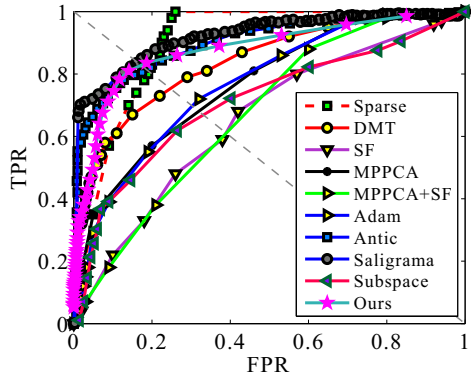
Figure 9. Frame-level comparison of the ROC curves in UCSD Ped1 dataset. Method abbreviation: MPPCA+SF [13], SF [13], MDT [13], Sparse [5], Saligrama [16], Antic [2], Subspace: replacing our combination learning by subspace clustering [7].
