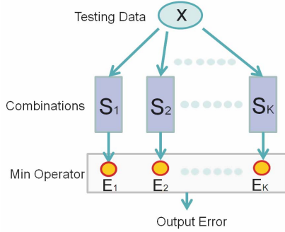
Figure 1. Our testing architecture. \mathbf{X} denotes testing data. \{\mathbf{S}_1, \dots, \mathbf{S}_K\} are learned combinations, with each \mathbf{S}_i \in \mathbb{R}^{p \times s} ( s \ll q ). E_i is the corresponding least square reconstruction error. The final error is the minimum among all combinations.
