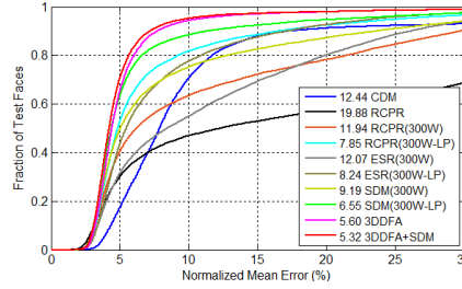
Figure 9. Comparisons of cumulative errors distribution (CED) curves on AFLW. To balance the pose distribution, we plot the CED curves with a subset of 12,081 samples whose absolute yaw angles within [0^\circ, 30^\circ] , [30^\circ, 60^\circ] and [60^\circ, 90^\circ] are 1/3 each.
