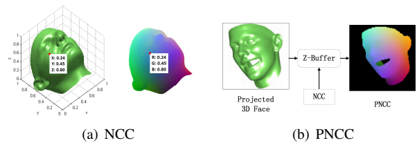
Figure 3. The Normalized Coordinate Code (NCC) and the Projected Normalized Coordinate Code (PNCC). (a) The normalized mean face, which is also demonstrated with NCC as its texture ( NCC_x = R , NCC_y = G , NCC_z = B ). (b) The generation of PNCC: The projected 3D face is rendered by Z-Buffer with NCC as its colormap.
