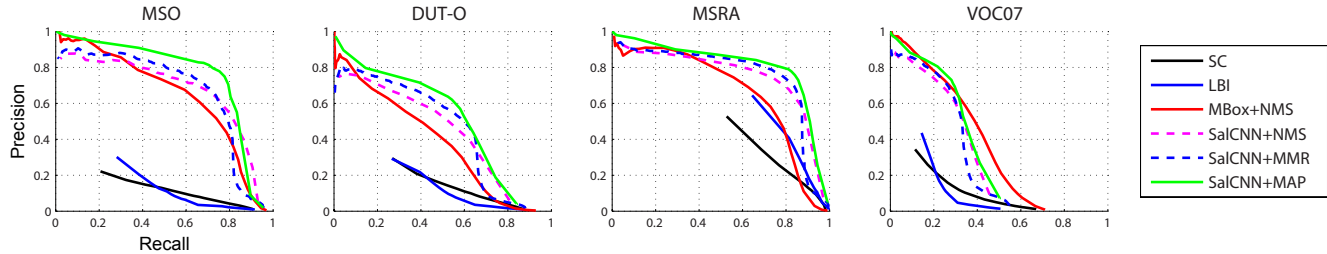
Figure 3: Precision-Recall curves. Our full method SalCNN+MAP significantly outperforms the other methods on MSO, DUT-O and MSRA. On VOC07, our method is slightly worse than MBox [46], but VOC07 is not a salient object dataset.
