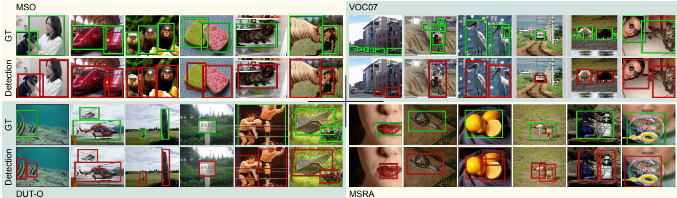
Figure 5: Sample detection results of our method when \lambda = 0.1 . In the VOC07 dataset, many background objects are annotated, but our method only detects dominant objects in the scene. In the DUT-O and MSRA datasets, some ground truth windows cover multiple objects, while our method tends to localize each object separately. Note that we are showing all the detection windows produced by our method. More detection results are included in the supplementary material.
