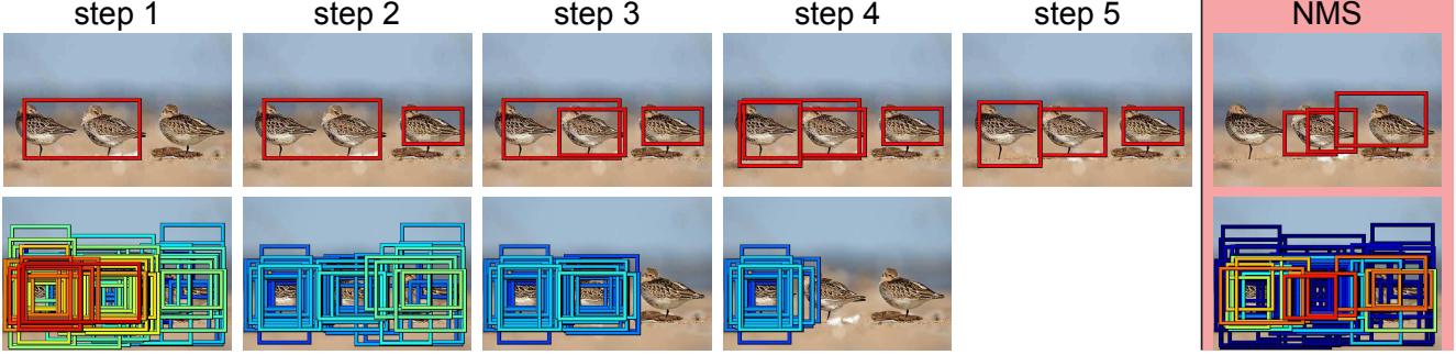
Figure 2: In column 1-5, we show step-by-step window selection results of our greedy algorithm. In the incrementing pass (step 1-4), windows are selected based on their marginal gains w.r.t. Eq. 11. The window proposals of positive marginal gains are shown in the bottom row for each step. Warmer colors indicate higher marginal gains. The final step (step 5) removes the first selected window in the decrementing pass, because our formulation favors a small number of detection windows with small inter-window overlap. To contrast our method with greedy NMS, we show the top 3 output windows after greedy NMS using an IOU threshold of 0.4 (top). The scored proposals are shown in the bottom row of the figure.
