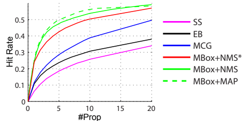
Figure 4: Object proposal generation performance (hit rate vs. average #Prop per image) on VOC07. Our MAP-based formulation further improves the state-of-the-art MBox method when #Prop is small.
