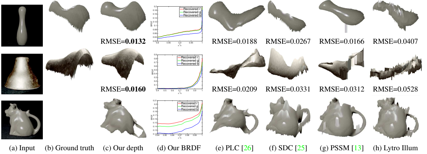
Figure 7: Shape and reflectance estimation results on real data with homogeneous BRDFs. The intensities of the input images are adjusted for better contrast. It can be seen that our method realistically reconstructs the shapes, and also achieves the lowest RMSE when ground truth is available. The recovered BRDFs also look qualitatively correct, e.g., the bowling pin has a very sharp specularity.
