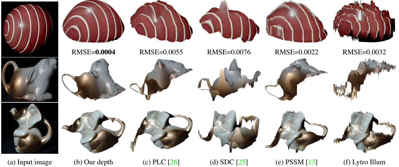
Figure 8: Shape estimation results on real data with spatially-varying BRDFs. It can be seen that our method realistically reconstructs the shapes, while other methods generate artifacts around the specular regions.
