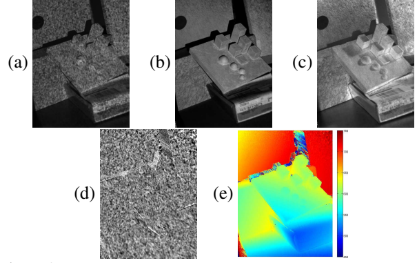
Figure 3. Left-to-right: a) I_c , b) coefficients a and c) b from Equation 2 for the MAP-estimated range d) I_p in the camera image plane, e) the range image in mm. Note how parameter b captures scene illumination, whereas parameter a captures the reflectance coefficient of the surface with respect to the projector.
