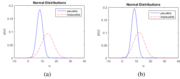
Figure 7: Gaussian distribution of d_{normal} for plausible (blue) and implausible (red) 3D reconstructions. For Evaluation 1 (Fig. 7a) the intersection is in u = 11.08 and for Evaluation 2 (Fig. 7b) it is in u = 10.95 .
