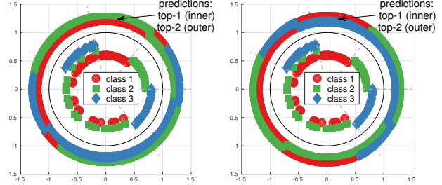
(a) top-1 \text{SVM}_1 test accuracy (top-1 / top-2): 65.7% / 81.3% (b) top-2 \text{Ent}_{\text{tr}} test accuracy (top-1 / top-2): 29.4% / 96.1%
