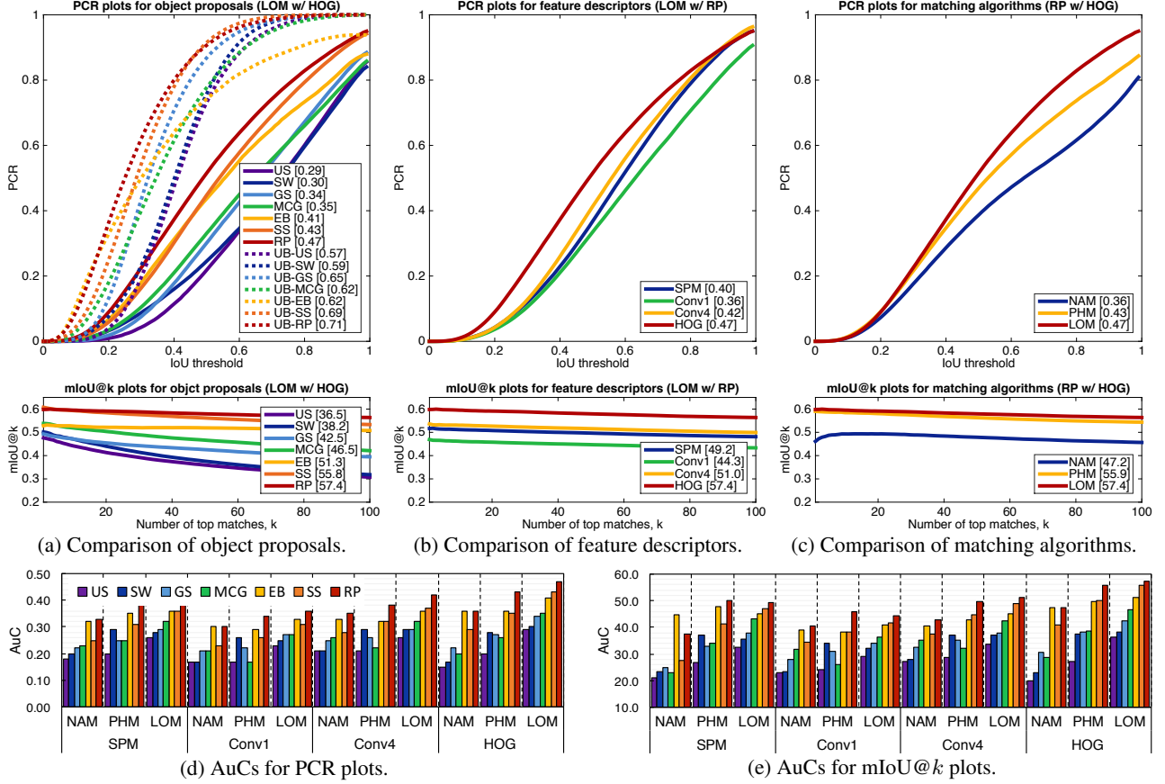
Figure 5. PF benchmark evaluation on (a-c) region matching precision (top, PCR plots) and match retrieval accuracy (bottom, mIoU@k plots), and (d-e) AuCs for different combinations of object proposals, feature descriptors, and matching algorithms: (a) Evaluation for LOM with HOG [11], (b) evaluation for LOM with RP [40], (c) evaluation for RP with HOG [11], (d) AuCs for PCR plots, and (e) AuCs for mIoU@k plots. The AuC is shown in the legend. (Best viewed in color.)
