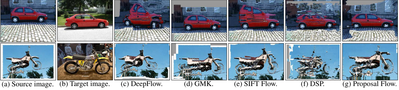
Figure 6. Examples of dense flow field. (a-b) Source images are warped to the target images using the dense correspondences estimated by (c) DeepFlow [46], (d) GMK [14], (e) SIFT Flow [35], (f) DSP [29], and (g) Proposal Flow (LOM w/ RP and HOG).
