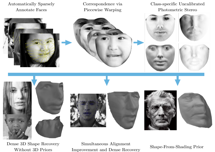
Figure 1: Illustrates the pipeline for construction and the uses of the model. The first row shows the rough model construction pipeline. The second row shows three uses demonstrated in the paper of the SH model.
