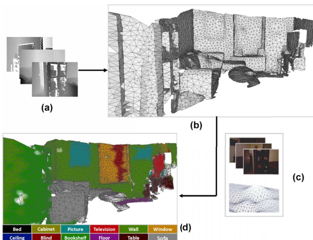
Figure 1. Semantic Mesh Segmentation: (a) shows the input to our system which is a sequence of images with depth estimates (here we show the images of a living room captured using a RGB-D camera [24]), (b) the depth estimates are used to generate a mesh based representation of the scene using the method of [31], (c) the system combines image level information and geometric contextual information from the mesh to perform object class labelling, (d) object class labelling is performed by establishing a conditional random field (CRF) on the mesh, with local neighbourhood interactions defined by the neighbouring faces in the mesh. (Best viewed in colour)
