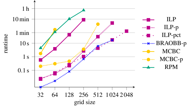
Figure 7. Average runtimes of those instances that could be solved in less than one hour (compare Fig. 8). For all methods reduction makes them applicable to larger instances. Overall, ILP-pct and BRAOBB-p perform best.
